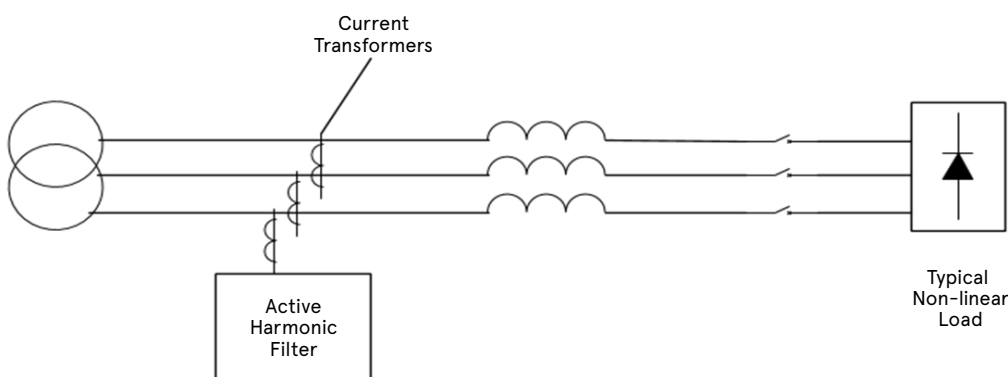
Figure 4: Active filter
