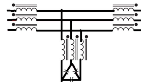
Figure 5: Passive filter
