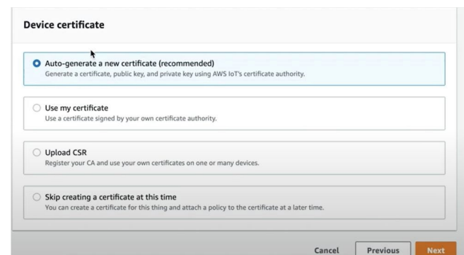
Fig 10: Generating certificates
