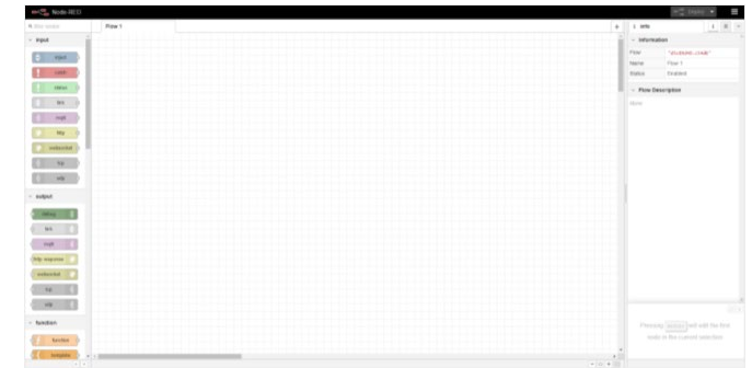
Fig5: Node-Red environment
