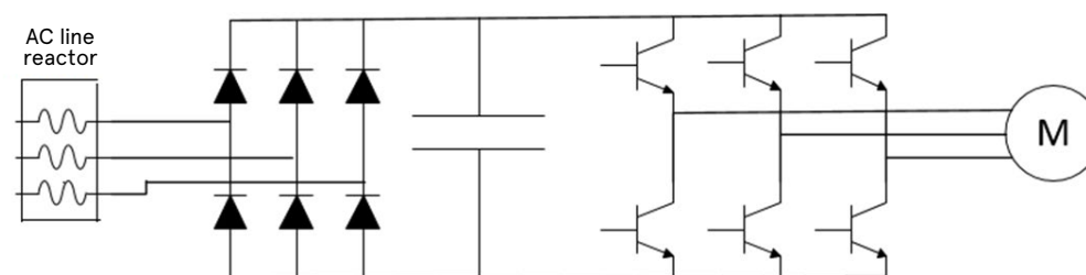
Figure 2: Line Reactors
